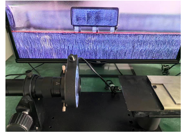
SMD骨架PIN平整度CDC检测
